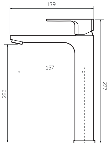
VISTA LATERAL / LATERAL VIEW
