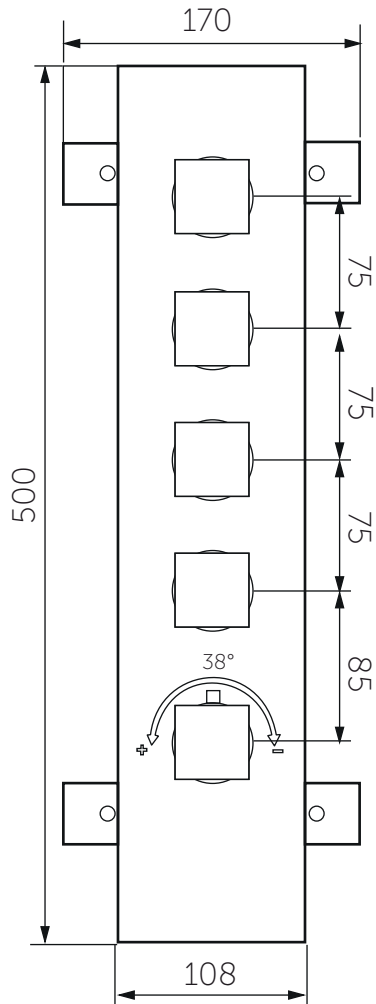
VISTA FRONTAL
